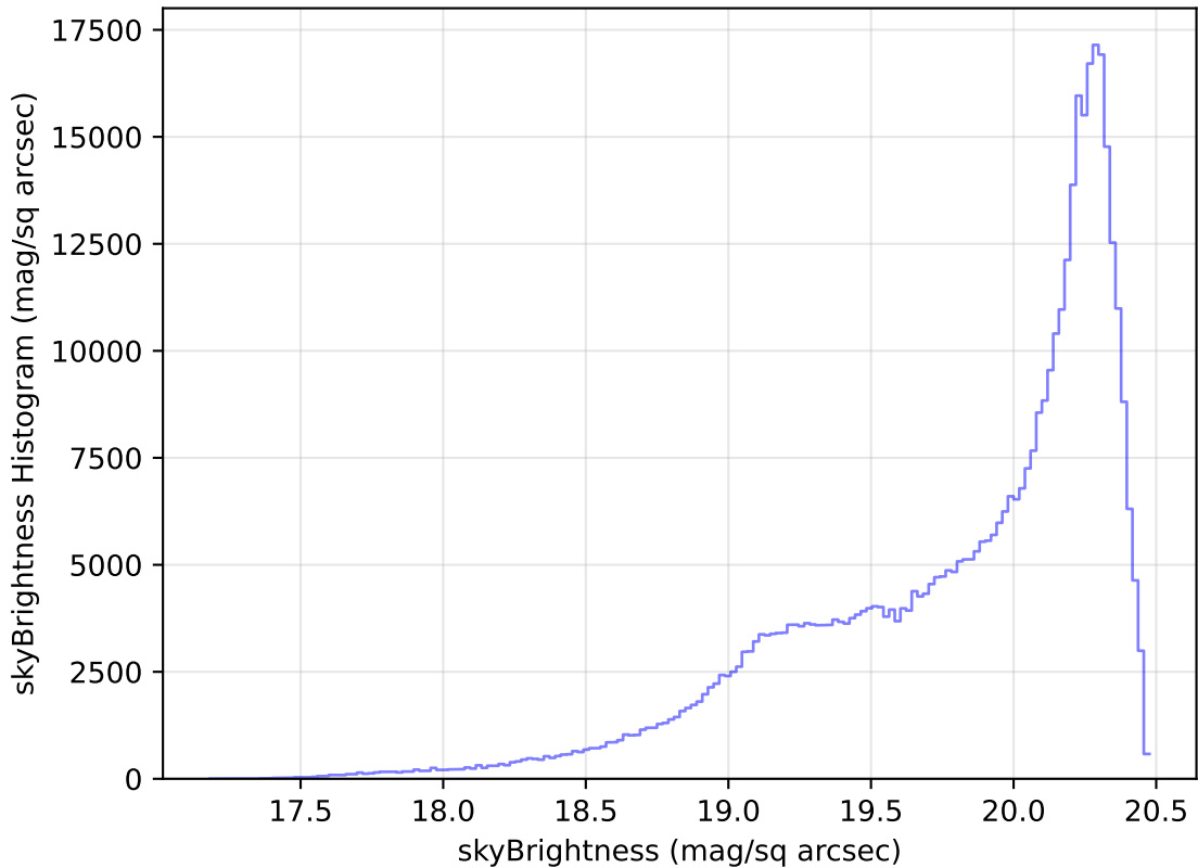
too_elab_r8_d2_gz_v3.4_10yrs All sky i band: skyBrightness Histogram
