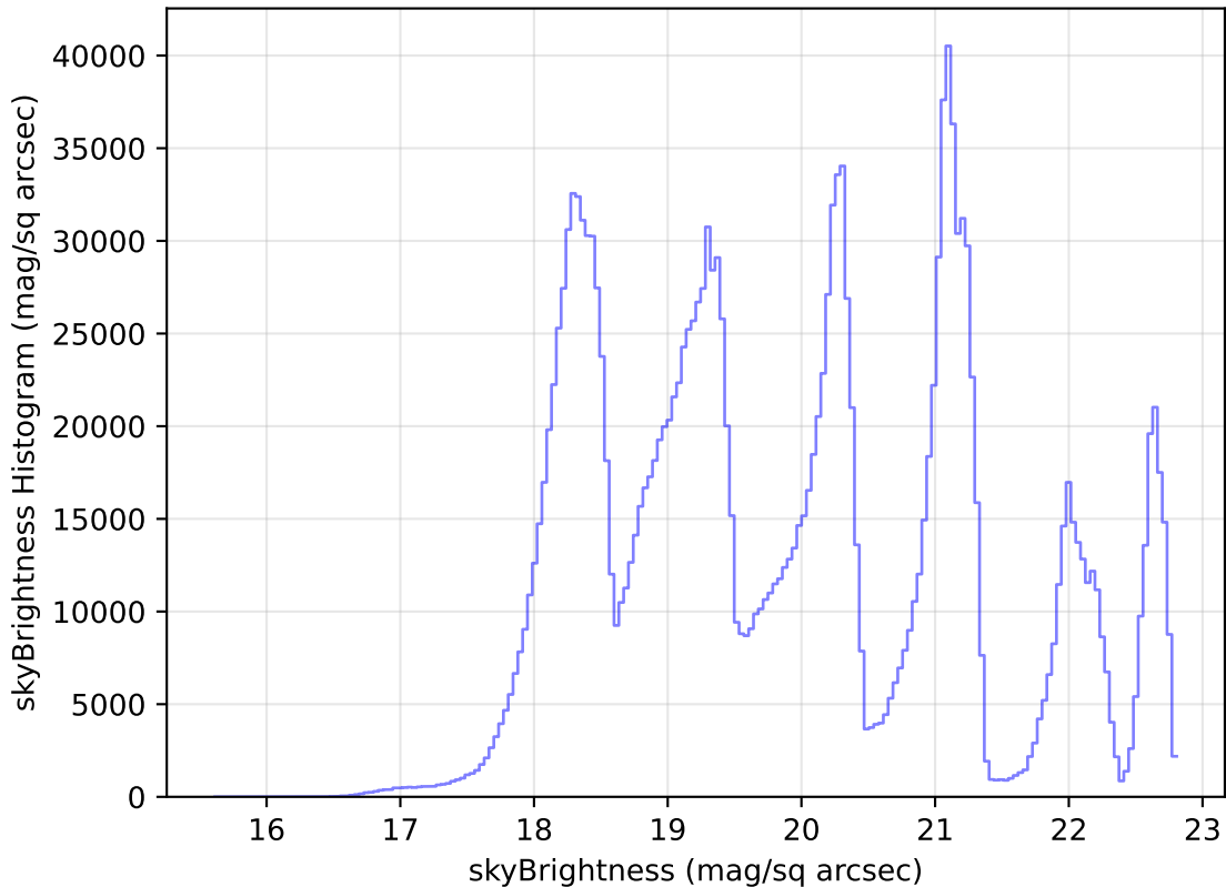
too_elab_r8_d2_gz_v3.4_10yrs All sky all bands: skyBrightness Histogram
