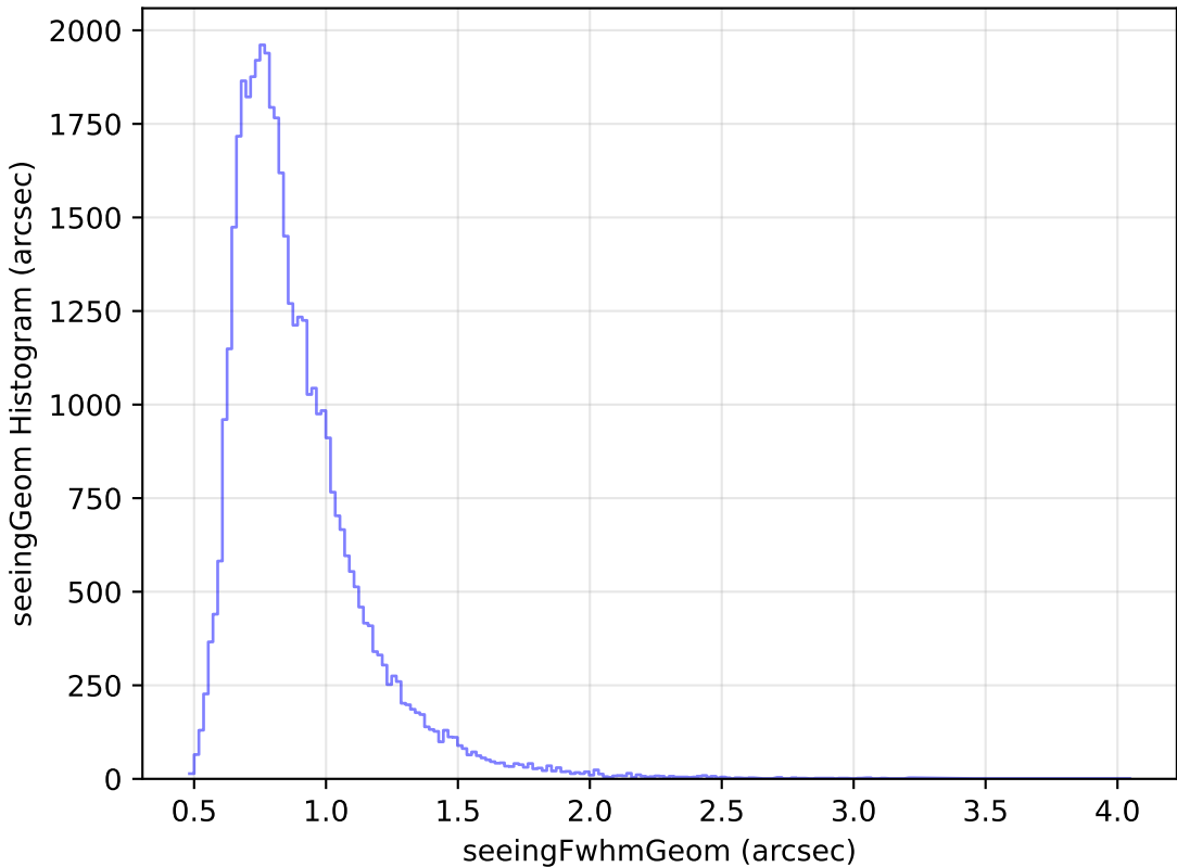
too_elab_r8_d2_gz_v3.4_10yrs Yr 1 z band: seeingGeom Histogram
