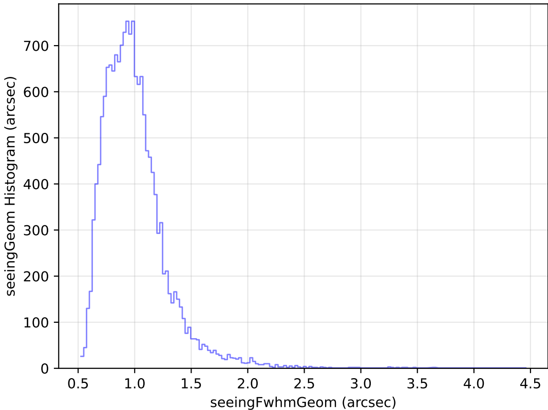
too_elab_r8_d2_gz_v3.4_10yrs Yr 1 u band: seeingGeom Histogram
