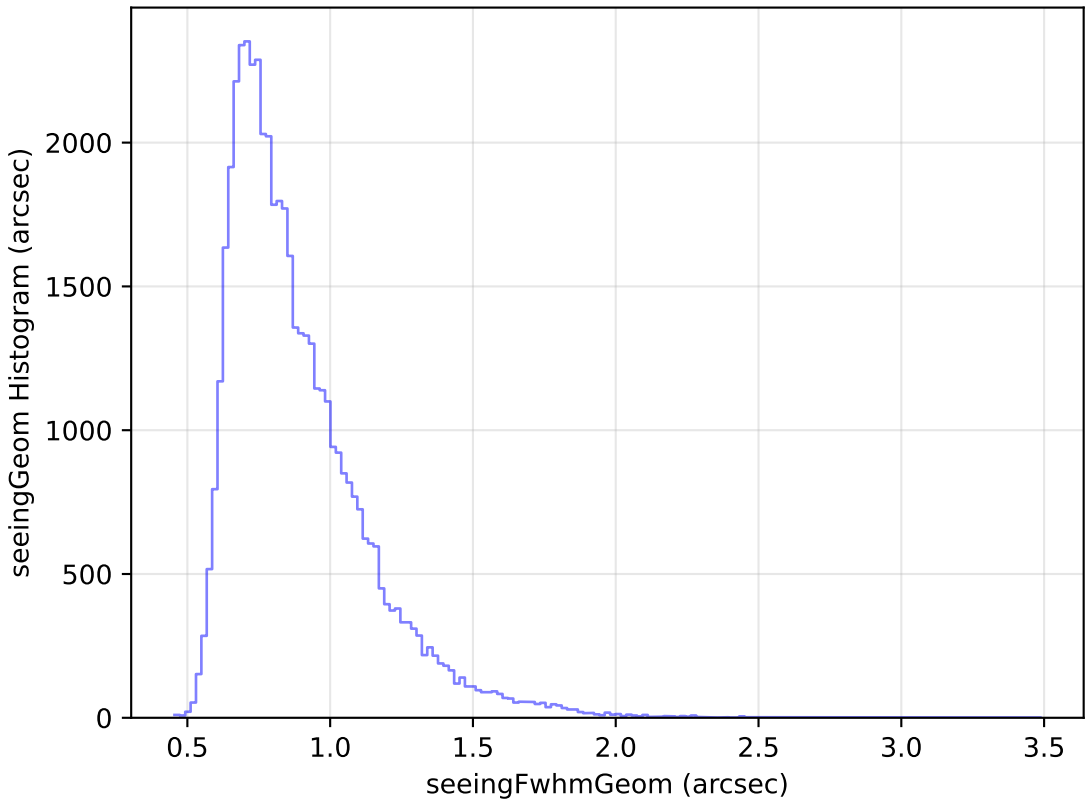
too_elab_r8_d2_gz_v3.4_10yrs Yr 1 r band: seeingGeom Histogram
