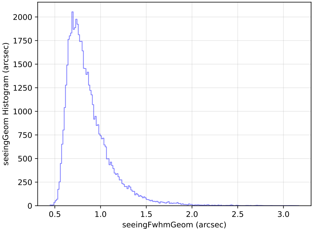
too_elab_r8_d2_gz_v3.4_10yrs Yr 1 i band: seeingGeom Histogram
