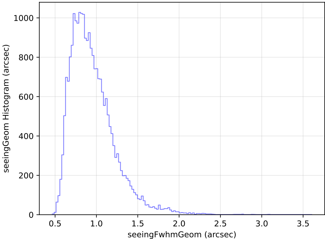
too_elab_r8_d2_gz_v3.4_10yrs Yr 1 g band: seeingGeom Histogram
