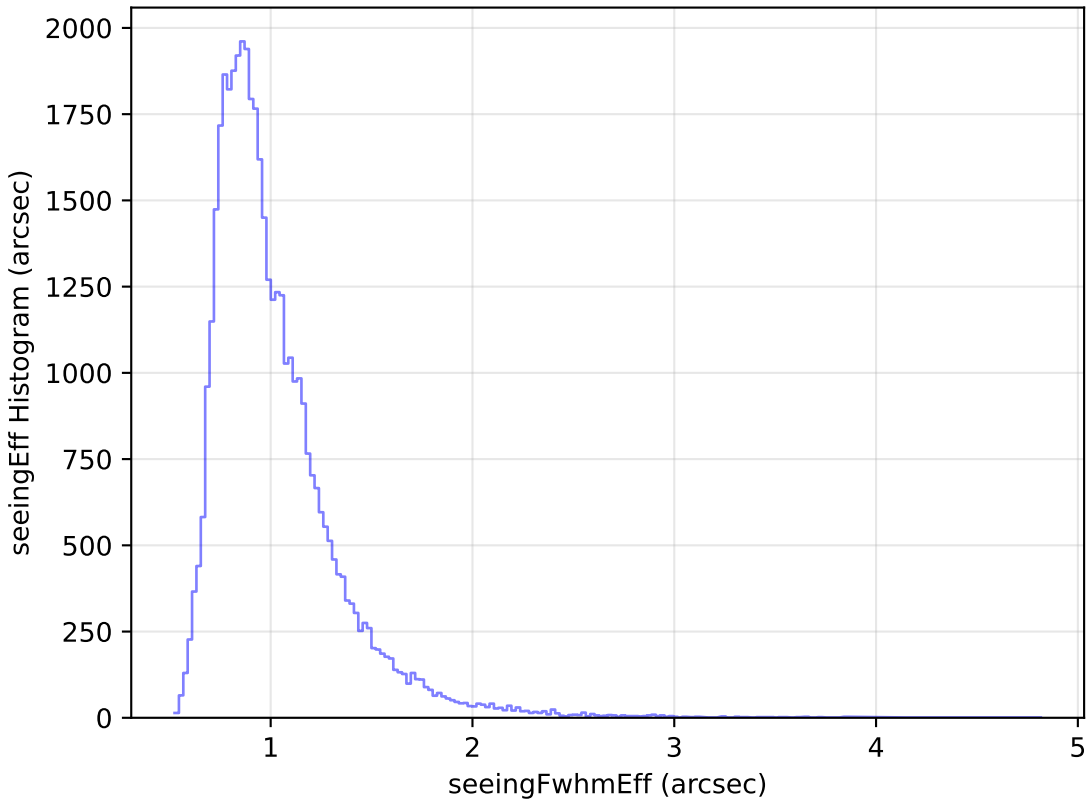
too_elab_r8_d2_gz_v3.4_10yrs Yr 1 z band: seeingEff Histogram
