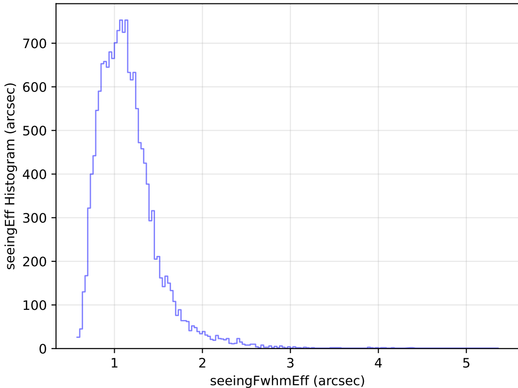
too_elab_r8_d2_gz_v3.4_10yrs Yr 1 u band: seeingEff Histogram
