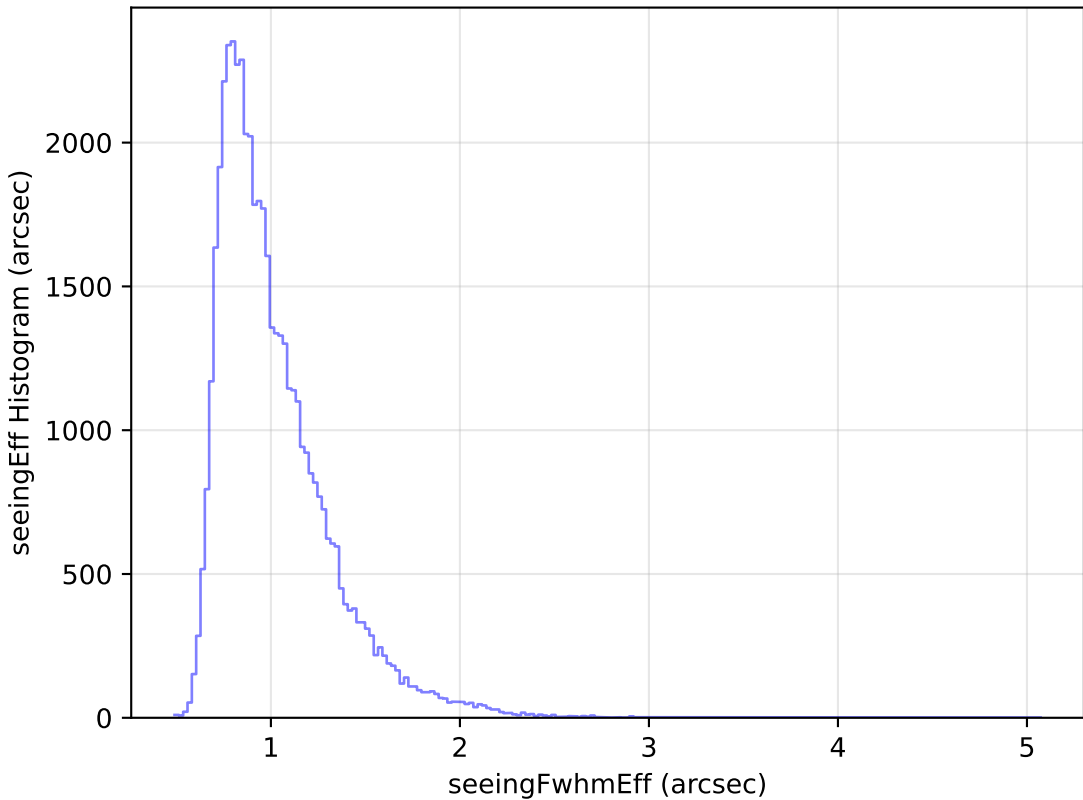
too_elab_r8_d2_gz_v3.4_10yrs Yr 1 r band: seeingEff Histogram
