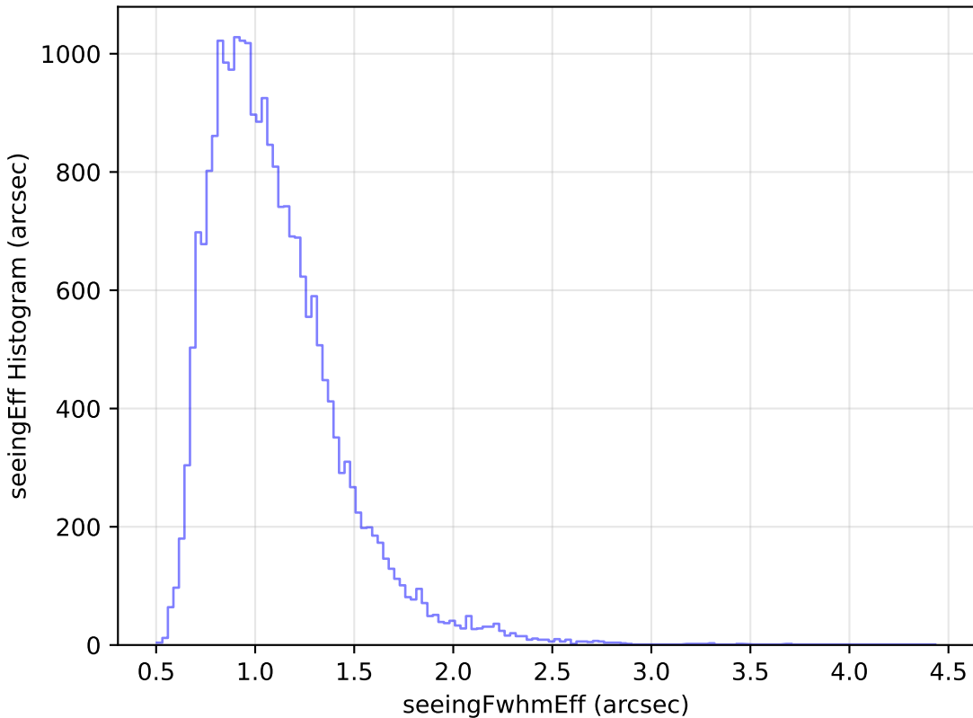
too_elab_r8_d2_gz_v3.4_10yrs Yr 1 g band: seeingEff Histogram
