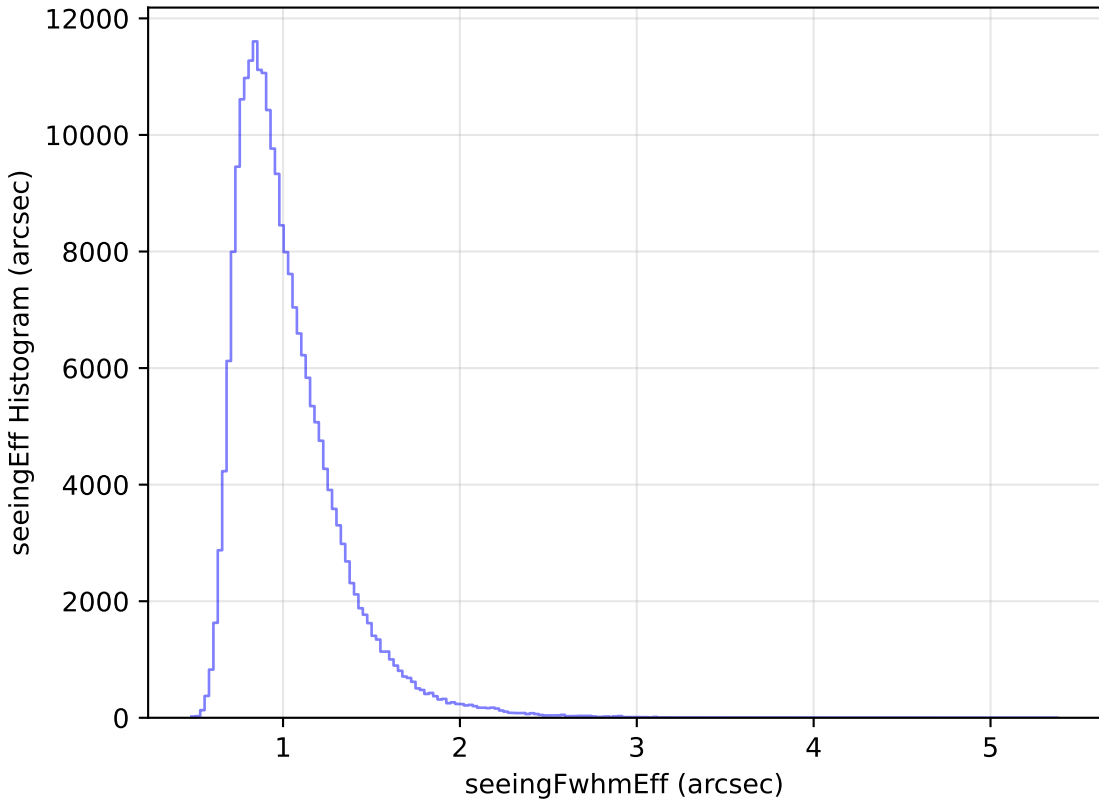
too_elab_r8_d2_gz_v3.4_10yrs Yr 1 all bands: seeingEff Histogram
