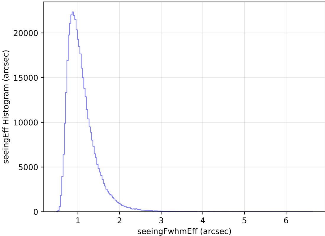
too_elab_r8_d2_gz_v3.4_10yrs WFD z band: seeingEff Histogram
