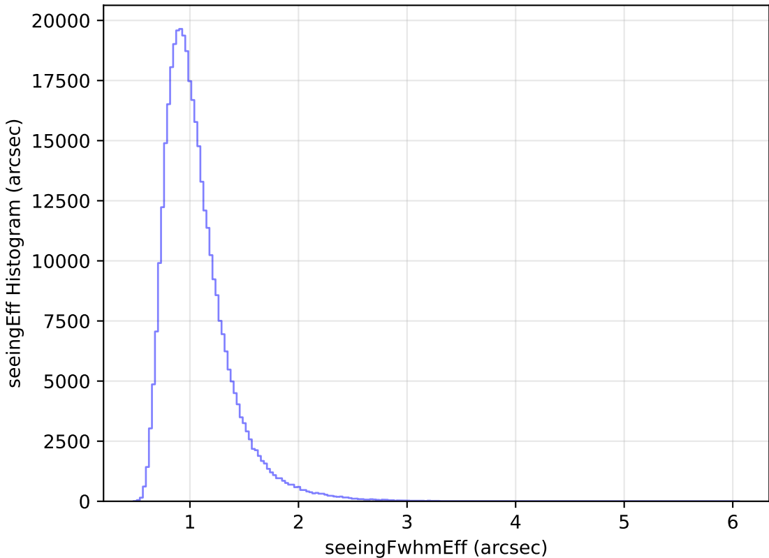
too_elab_r8_d2_gz_v3.4_10yrs WFD y band: seeingEff Histogram
