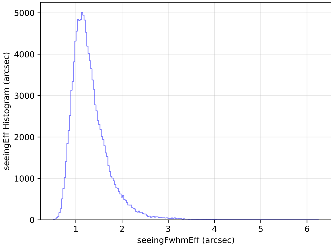
too_elab_r8_d2_gz_v3.4_10yrs WFD u band: seeingEff Histogram
