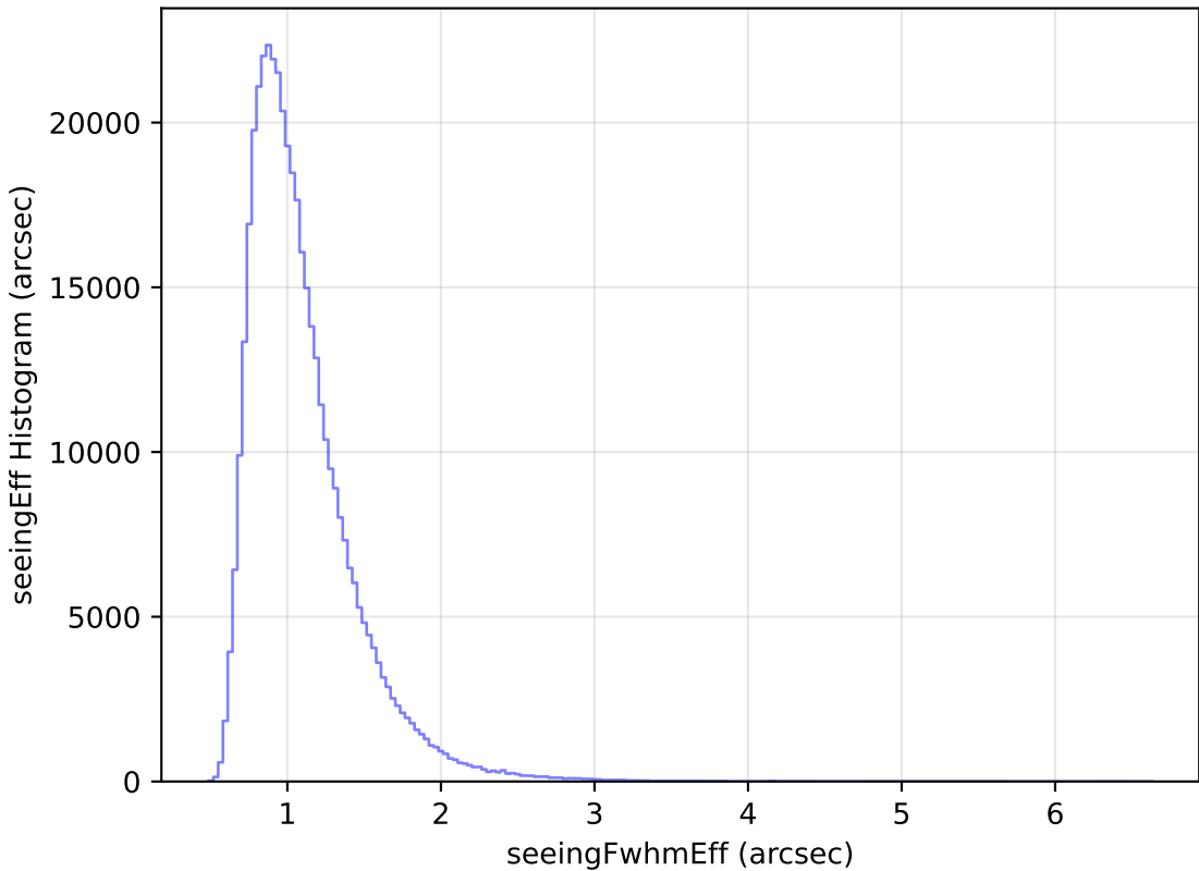
too_elab_r8_d2_gz_v3.4_10yrs All sky z band: seeingEff Histogram
