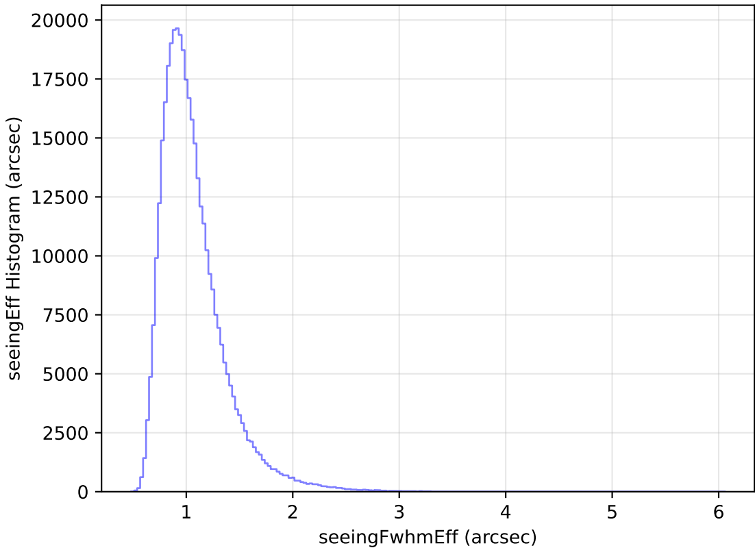
too_elab_r8_d2_gz_v3.4_10yrs All sky y band: seeingEff Histogram
