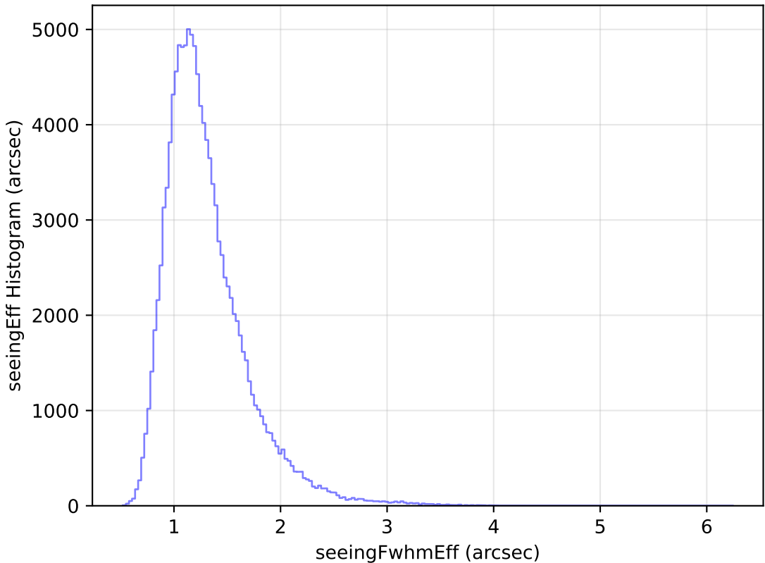
too_elab_r8_d2_gz_v3.4_10yrs All sky u band: seeingEff Histogram
