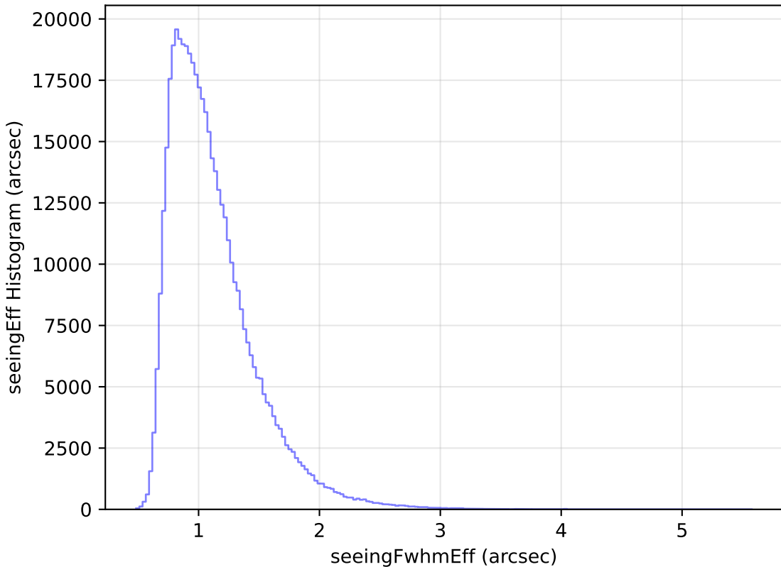
too_elab_r8_d2_gz_v3.4_10yrs All sky r band: seeingEff Histogram
