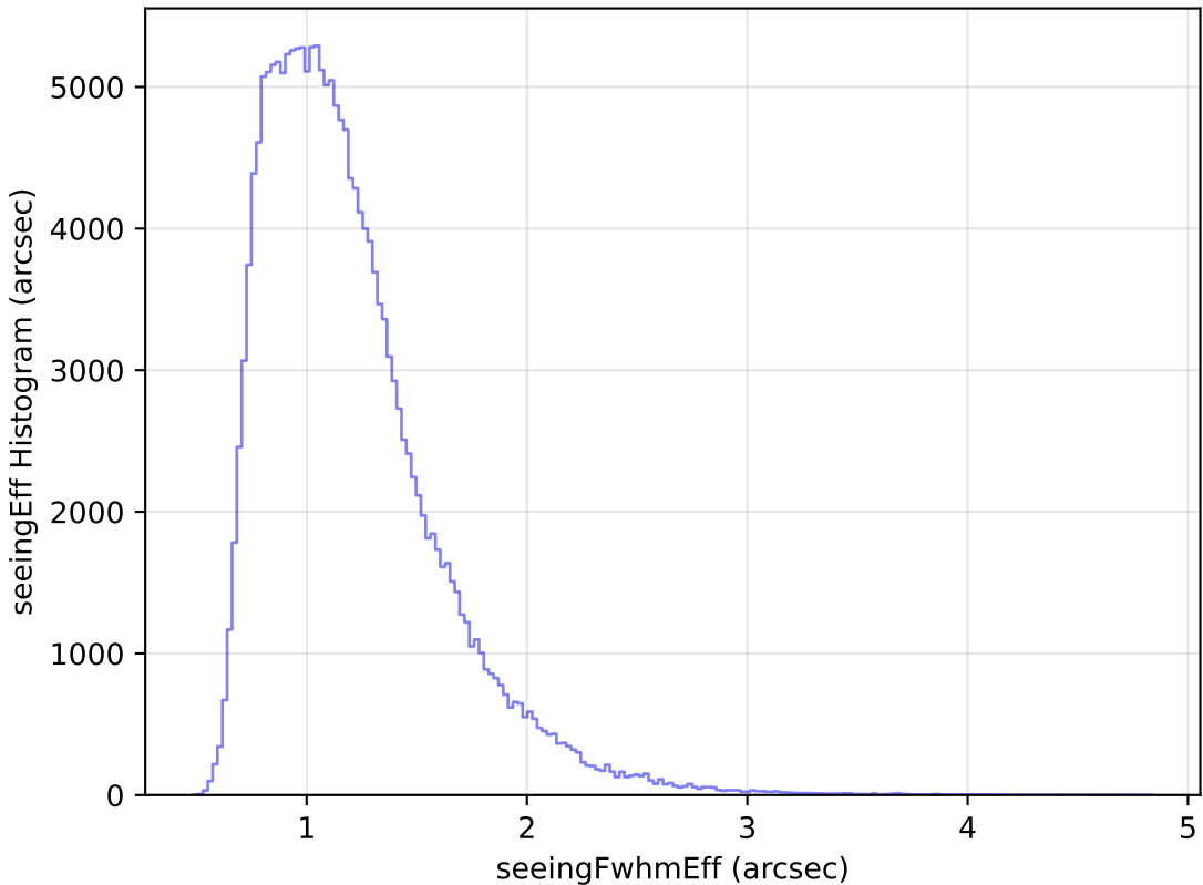
too_elab_r8_d2_gz_v3.4_10yrs All sky g band: seeingEff Histogram
