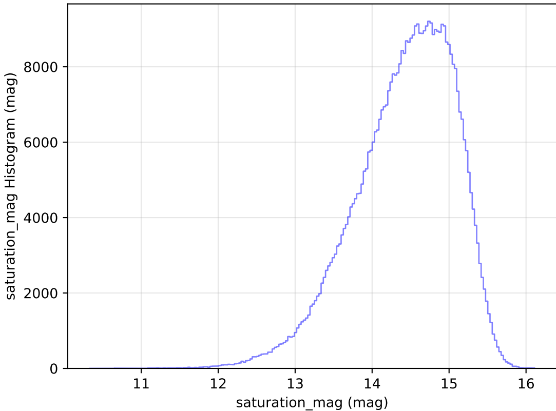
too_elab_r8_d2_gz_v3.4_10yrs WFD i band: saturation_mag Histogram
