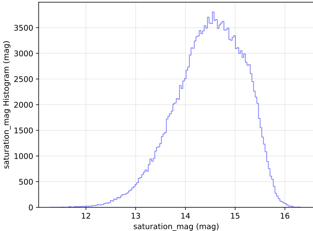
too_elab_r8_d2_gz_v3.4_10yrs WFD g band: saturation_mag Histogram
