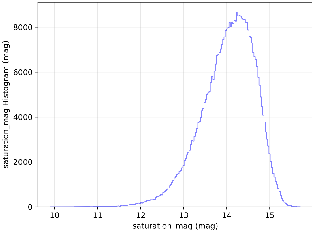
too_elab_r8_d2_gz_v3.4_10yrs All sky z band: saturation_mag Histogram
