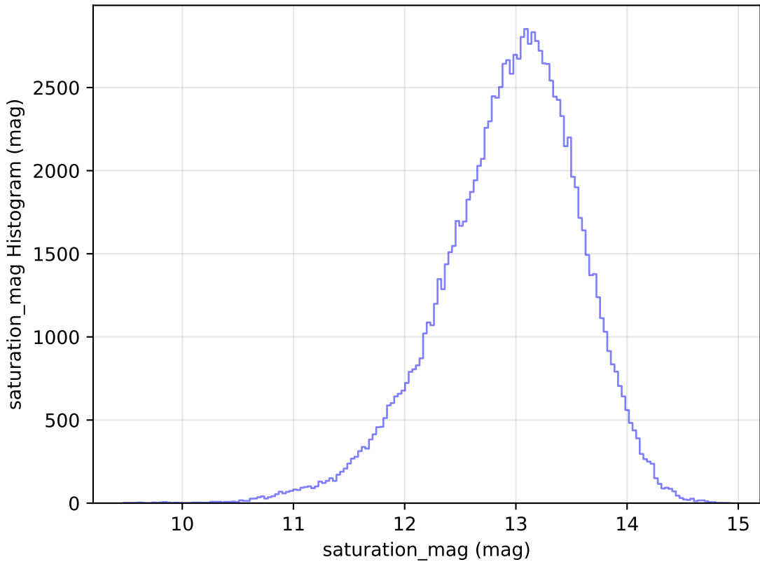
too_elab_r8_d2_gz_v3.4_10yrs All sky u band: saturation_mag Histogram
