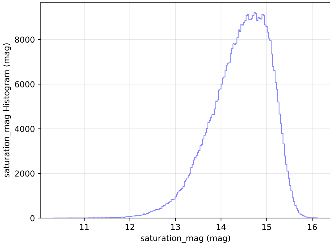
too_elab_r8_d2_gz_v3.4_10yrs All sky i band: saturation_mag Histogram
