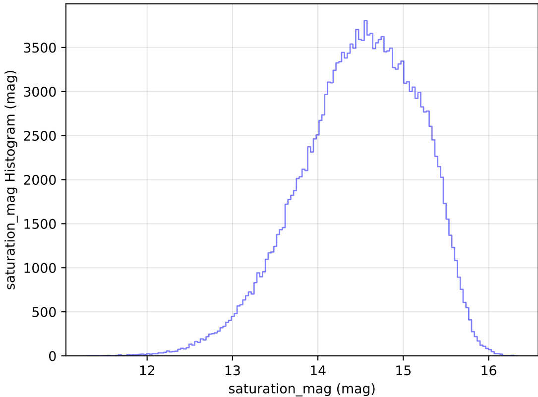
too_elab_r8_d2_gz_v3.4_10yrs All sky g band: saturation_mag Histogram
