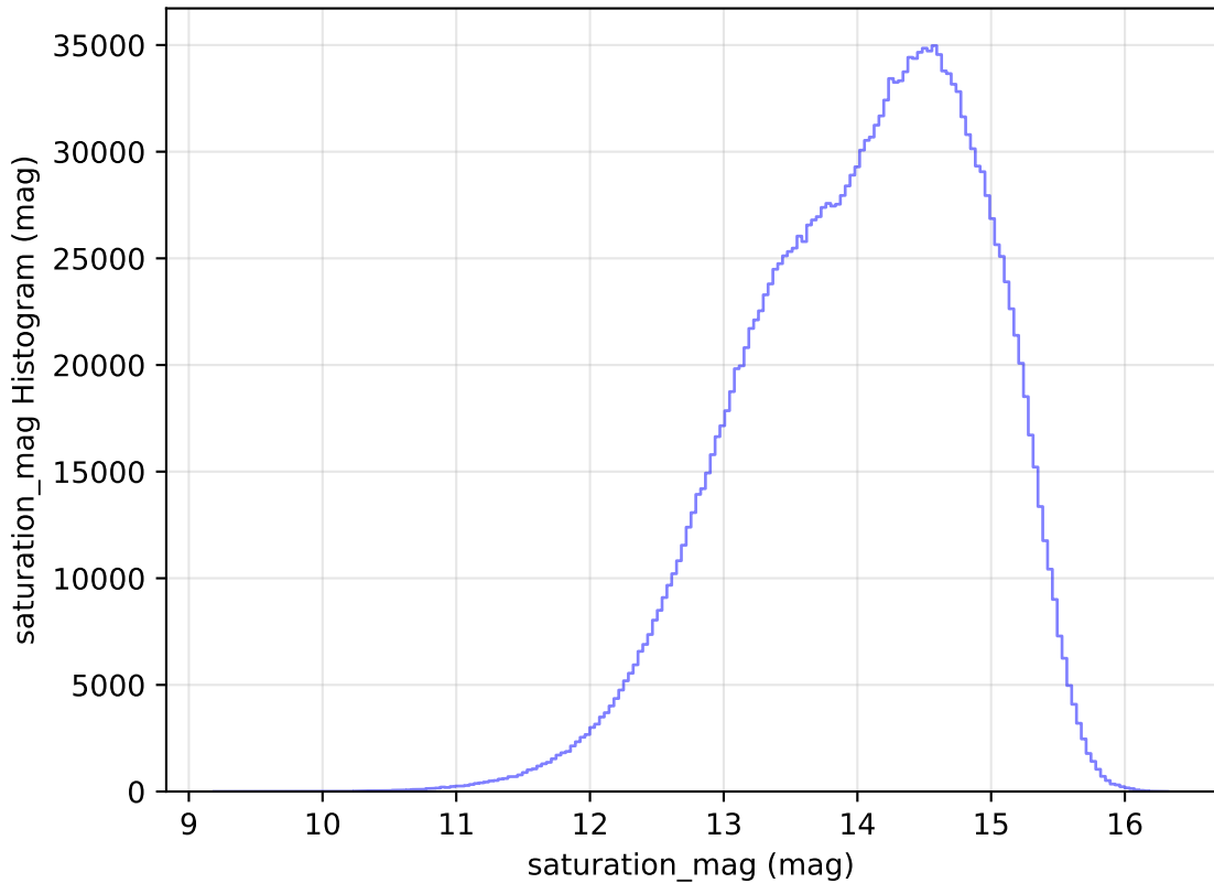
too_elab_r8_d2_gz_v3.4_10yrs All sky all bands: saturation_mag Histogram
