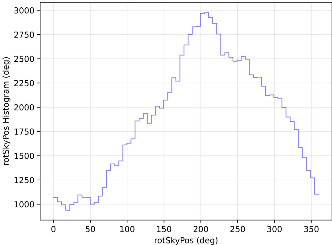
too_elab_r8_d2_gz_v3.4_10yrs WFD u band: rotSkyPos Histogram
