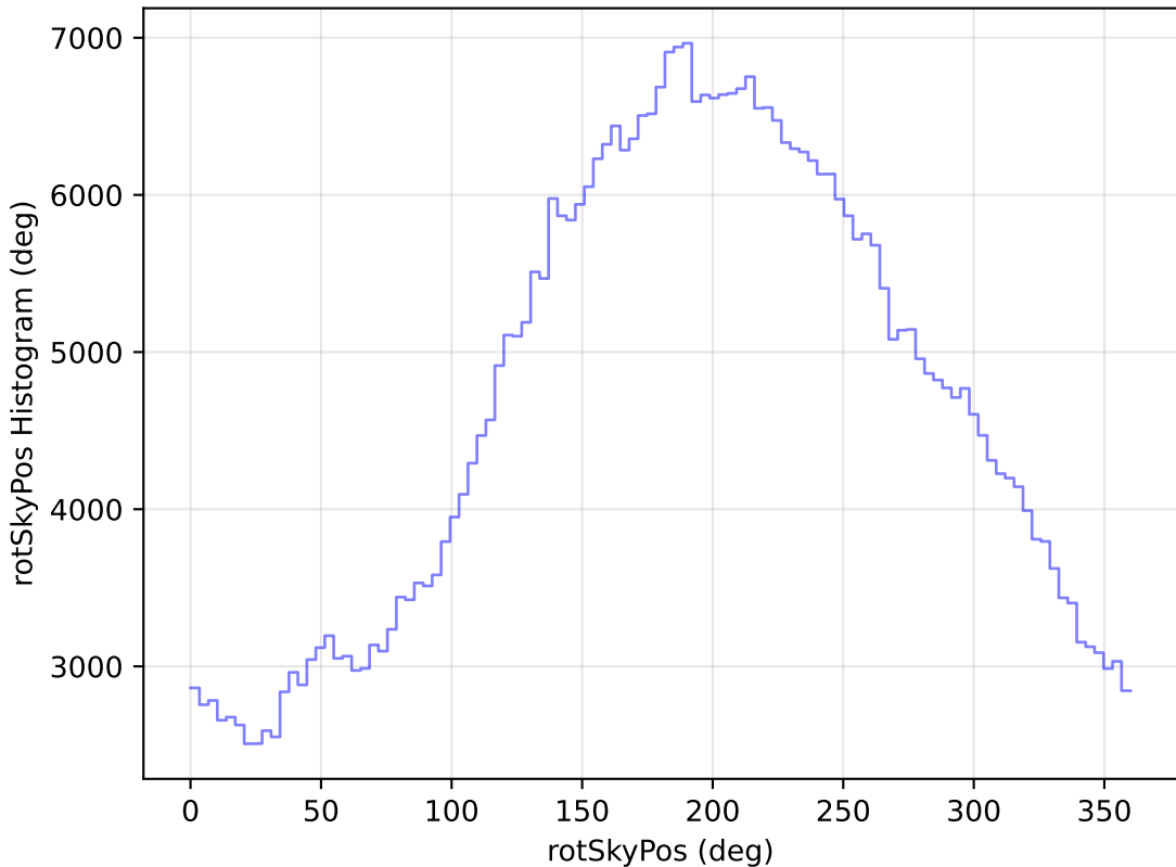
too_elab_r8_d2_gz_v3.4_10yrs WFD r band: rotSkyPos Histogram
