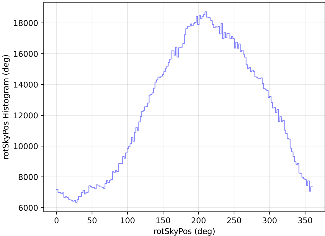
too_elab_r8_d2_gz_v3.4_10yrs WFD all bands: rotSkyPos Histogram
