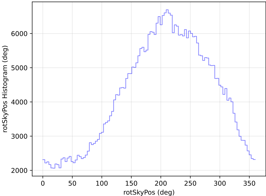
too_elab_r8_d2_gz_v3.4_10yrs All sky z band: rotSkyPos Histogram
