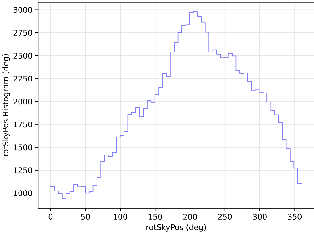
too_elab_r8_d2_gz_v3.4_10yrs All sky u band: rotSkyPos Histogram
