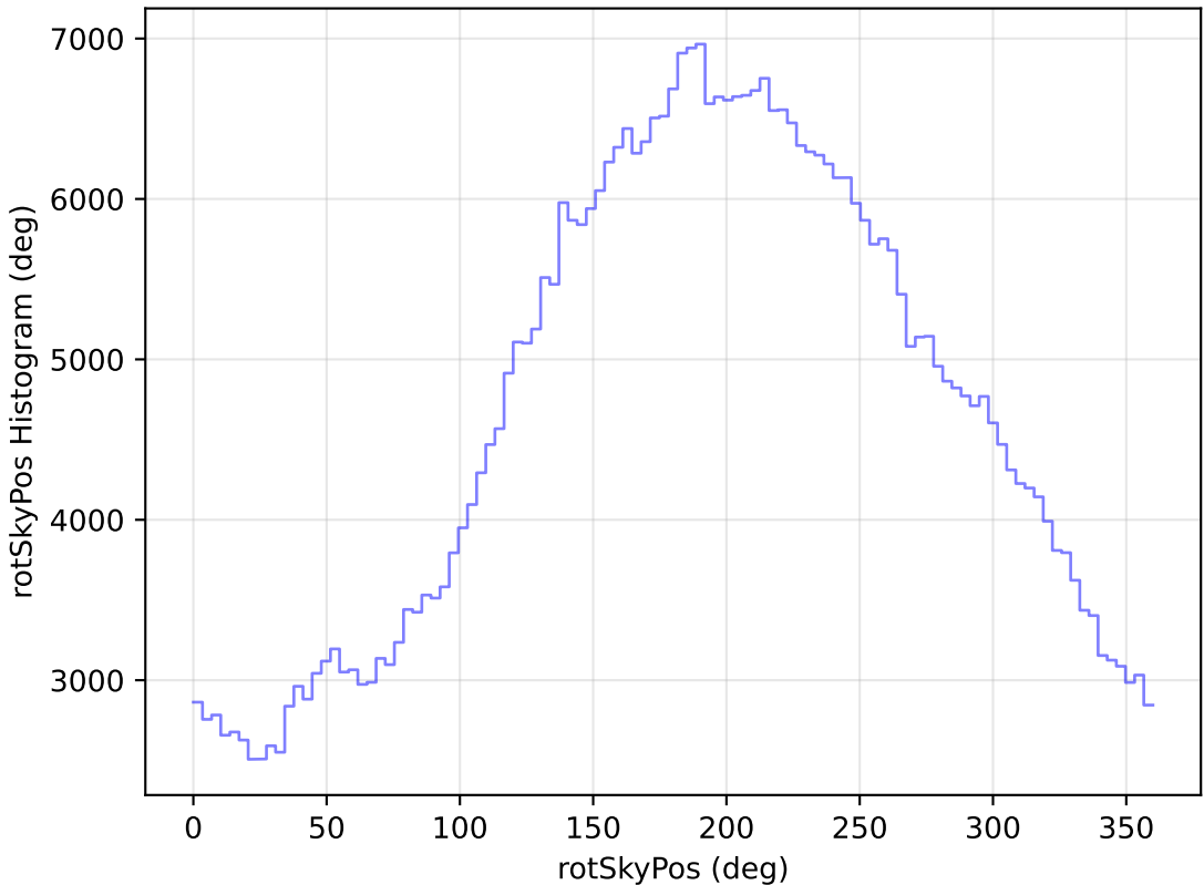
too_elab_r8_d2_gz_v3.4_10yrs All sky r band: rotSkyPos Histogram
