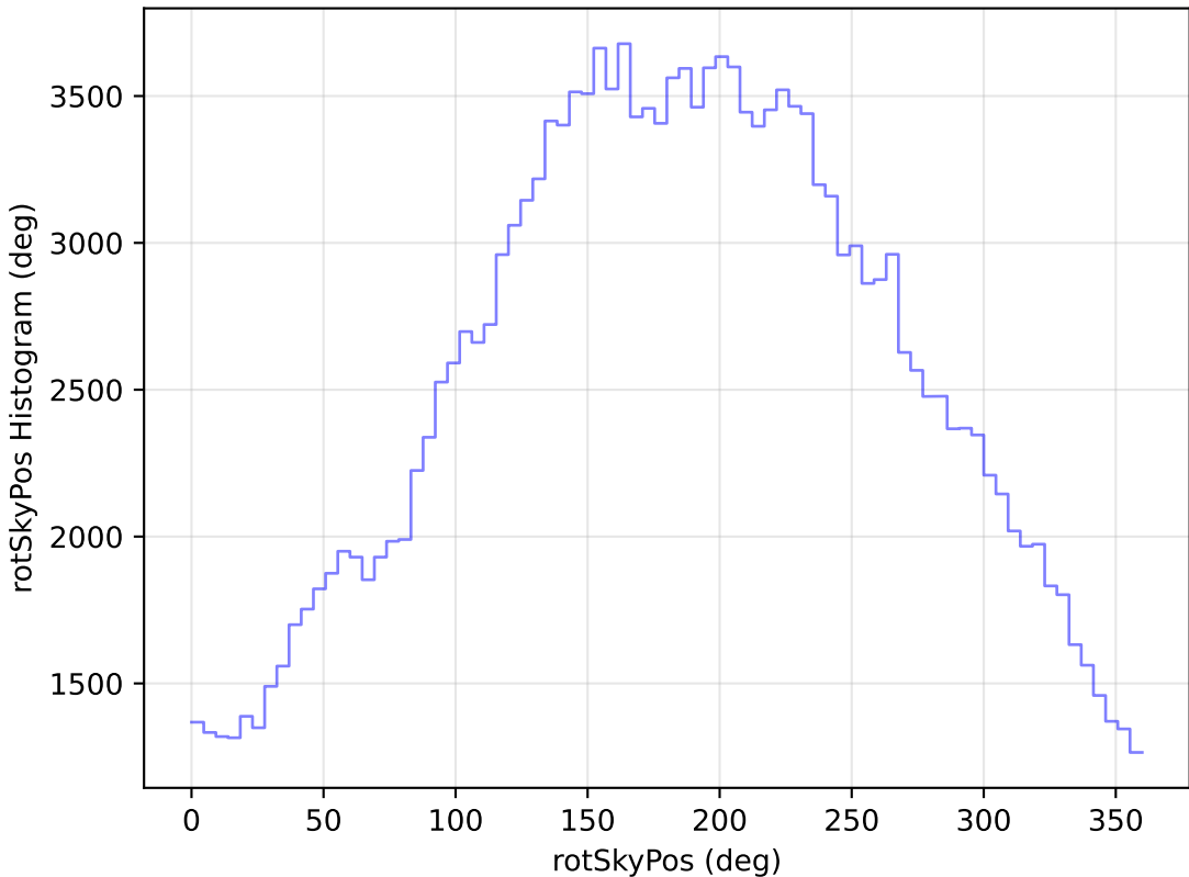
too_elab_r8_d2_gz_v3.4_10yrs All sky g band: rotSkyPos Histogram
