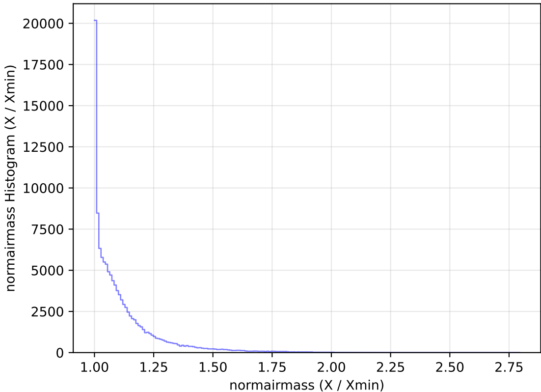
too_elab_r8_d2_gz_v3.4_10yrs WFD u band: normairmass Histogram
