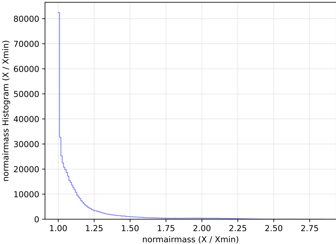
too_elab_r8_d2_gz_v3.4_10yrs WFD r band: normairmass Histogram
