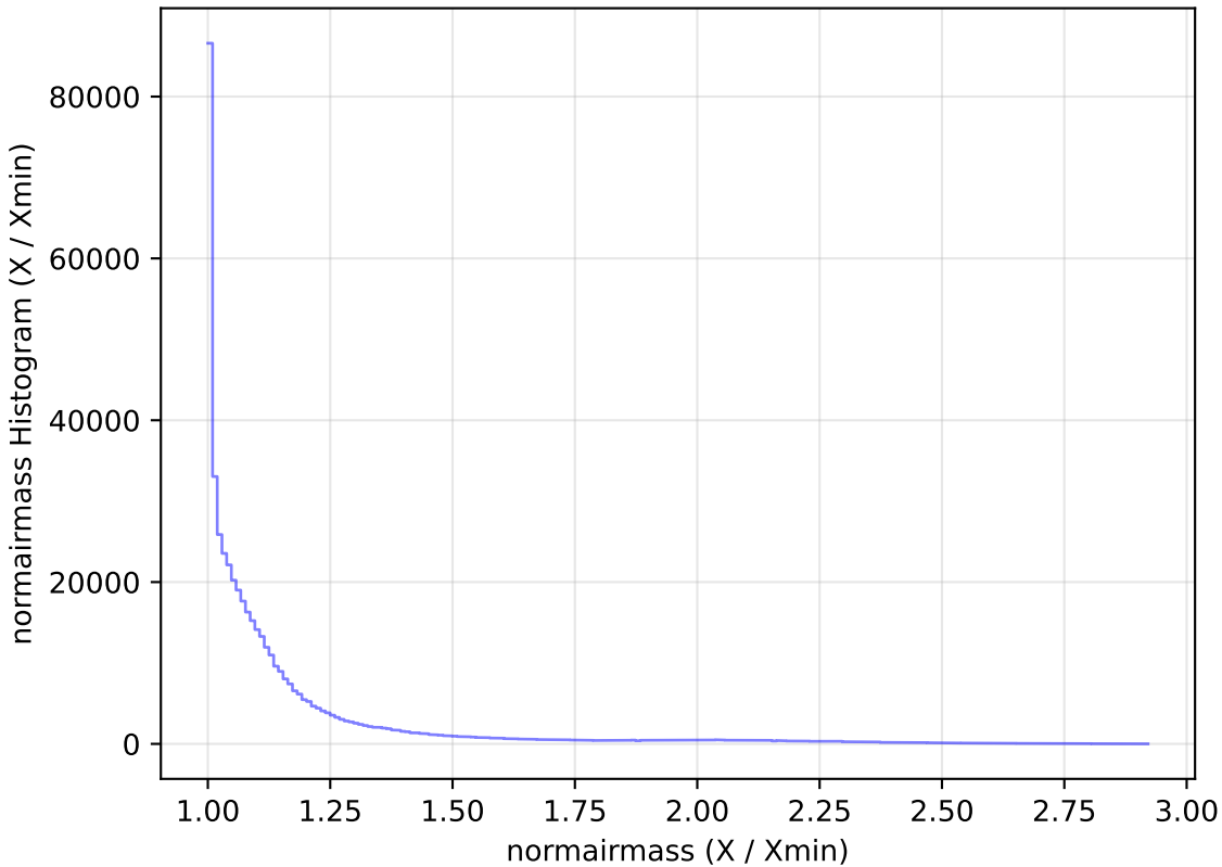
too_elab_r8_d2_gz_v3.4_10yrs WFD i band: normairmass Histogram
