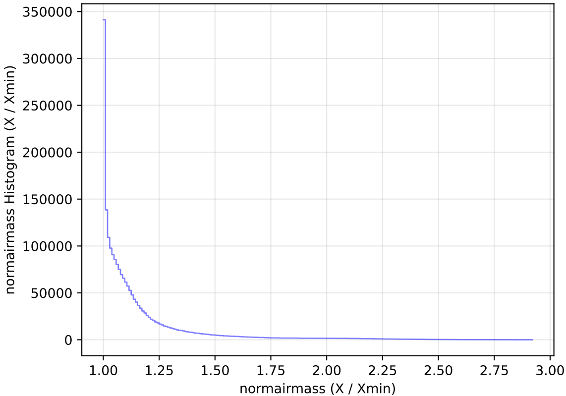
too_elab_r8_d2_gz_v3.4_10yrs WFD all bands: normairmass Histogram
