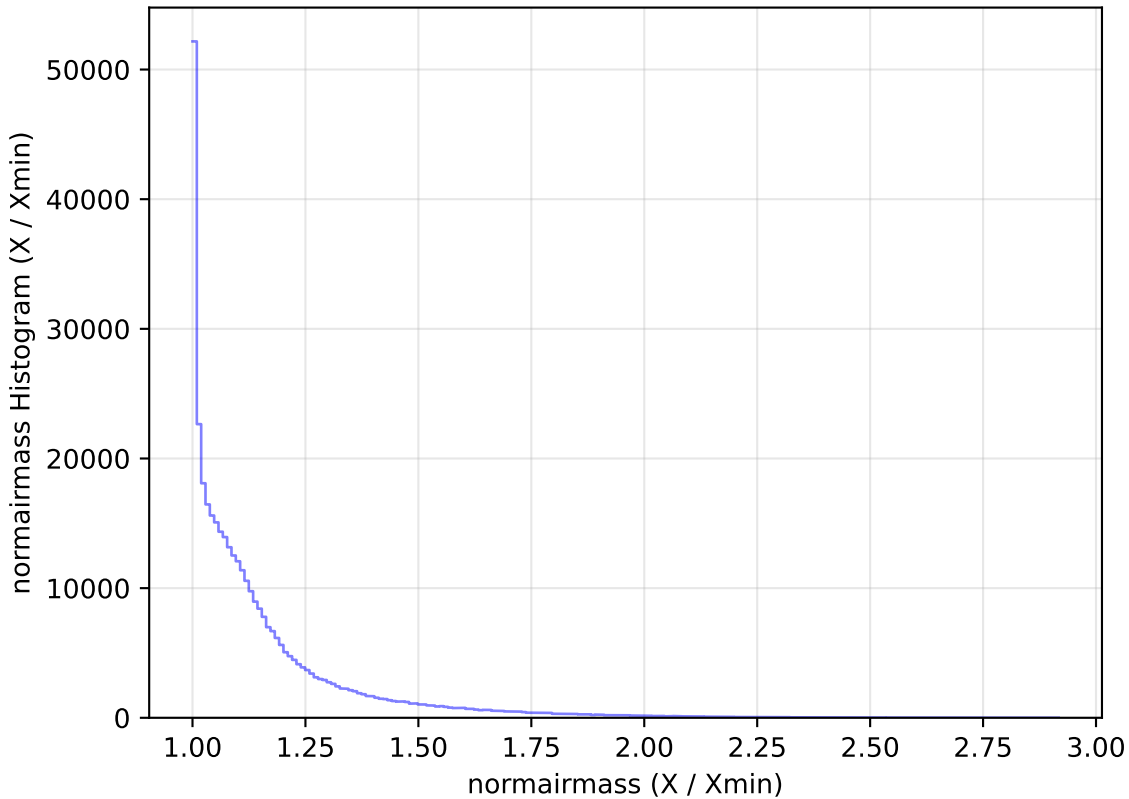
too_elab_r8_d2_gz_v3.4_10yrs All sky y band: normairmass Histogram
