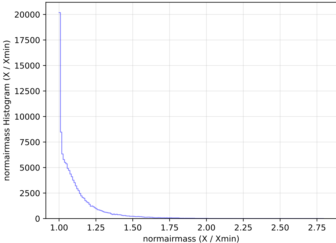
too_elab_r8_d2_gz_v3.4_10yrs All sky u band: normairmass Histogram
