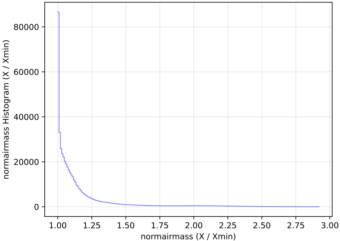
too_elab_r8_d2_gz_v3.4_10yrs All sky i band: normairmass Histogram
