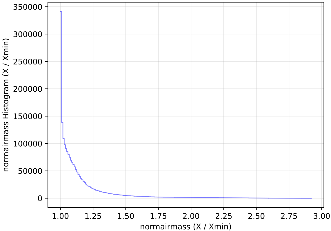
too_elab_r8_d2_gz_v3.4_10yrs All sky all bands: normairmass Histogram
