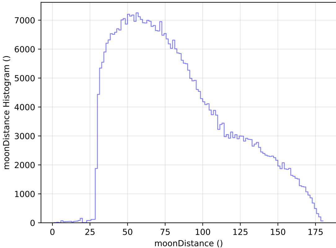
too_elab_r8_d2_gz_v3.4_10yrs WFD z band: moonDistance Histogram
