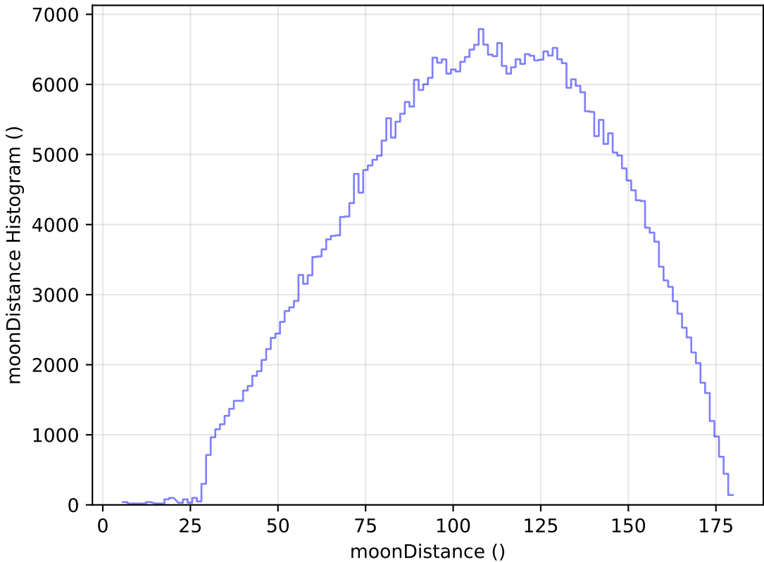
too_elab_r8_d2_gz_v3.4_10yrs WFD r band: moonDistance Histogram
