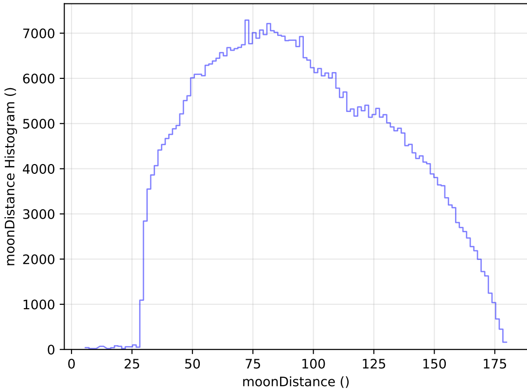
too_elab_r8_d2_gz_v3.4_10yrs WFD i band: moonDistance Histogram
