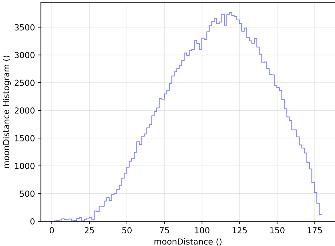
too_elab_r8_d2_gz_v3.4_10yrs WFD g band: moonDistance Histogram
