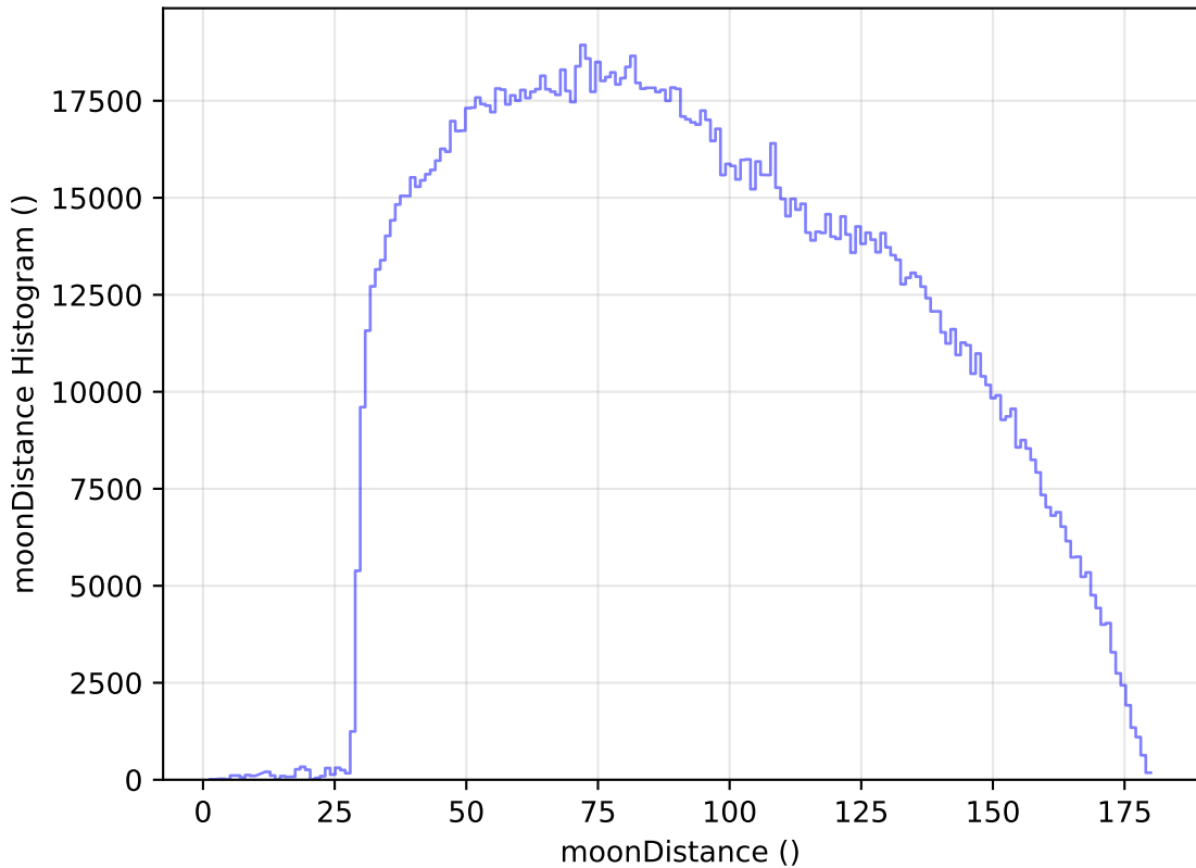
too_elab_r8_d2_gz_v3.4_10yrs WFD all bands: moonDistance Histogram
