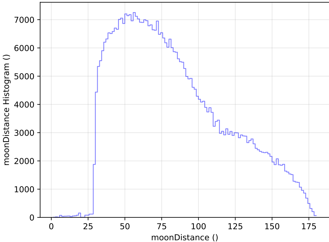
too_elab_r8_d2_gz_v3.4_10yrs All sky z band: moonDistance Histogram
