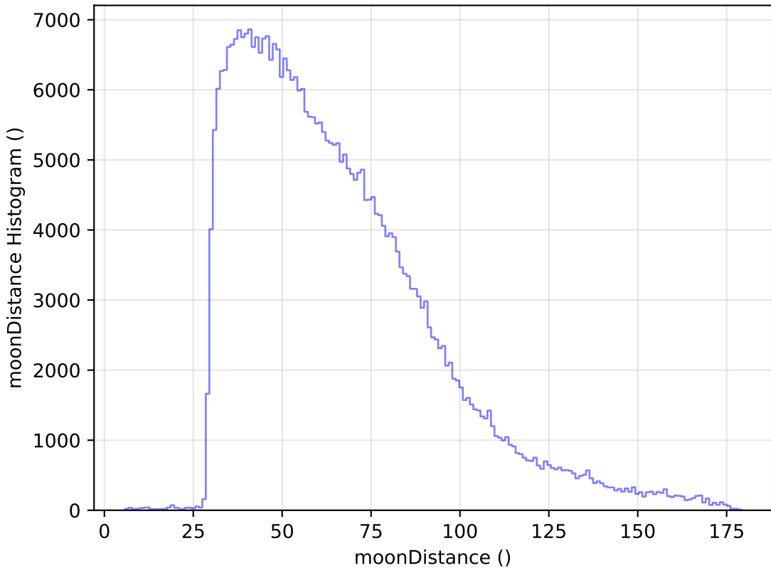
too_elab_r8_d2_gz_v3.4_10yrs All sky y band: moonDistance Histogram
