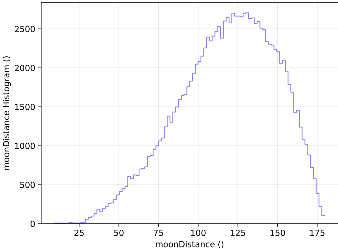
too_elab_r8_d2_gz_v3.4_10yrs All sky u band: moonDistance Histogram
